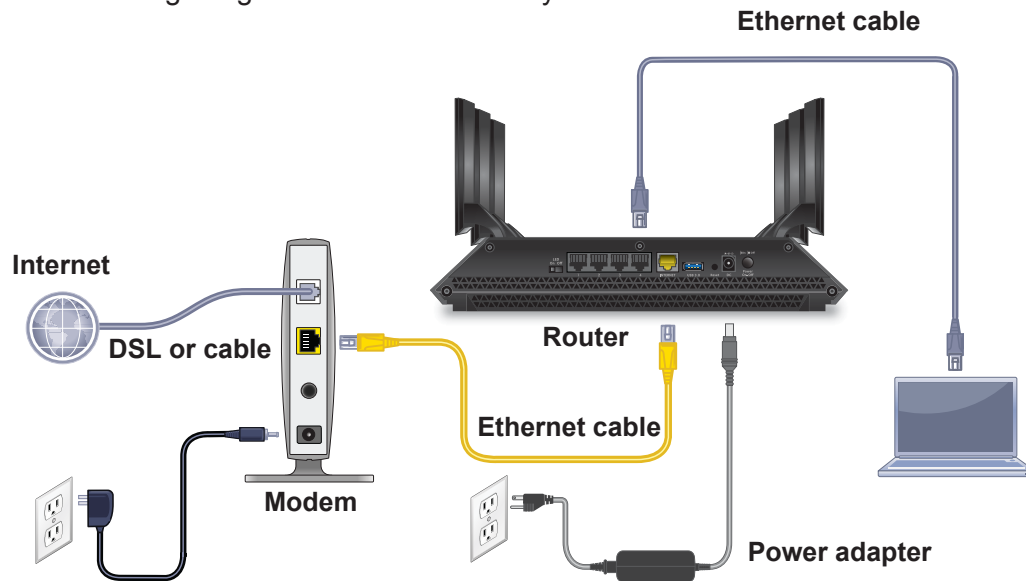
Figure 4. Router cabling
